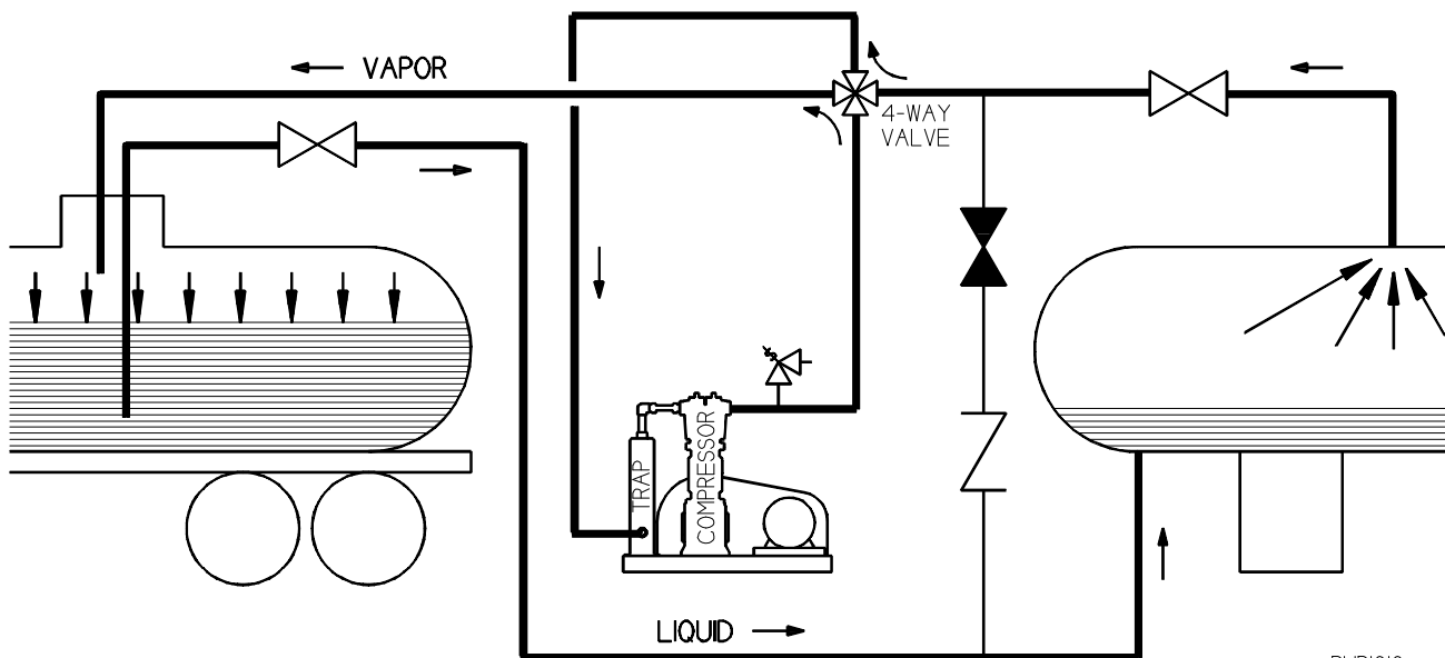
LIQUID TRANSFER
