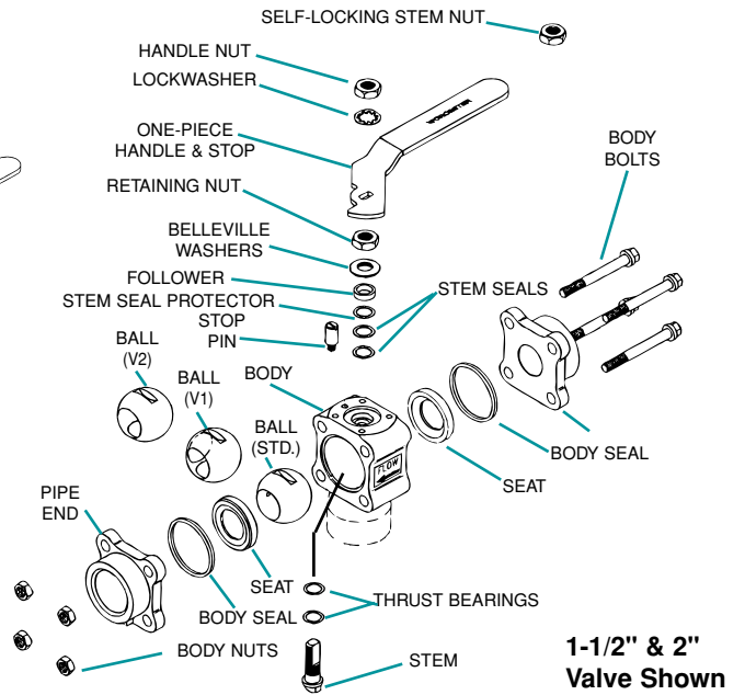
1/4" - 2" Cryogenic C44 and C44 Diverter Valves without Extension
